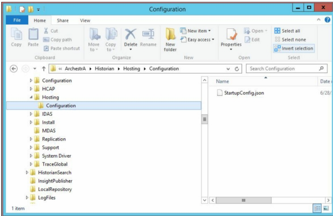
Figure 1: StartupConfig.json File
